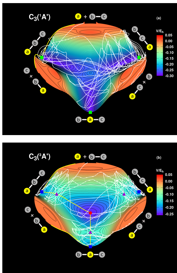
Fig. 2. Relaxed 3D plots in hyperspherical coordinates (Varandas 1987) of the nuclear-mass-independent PESs of ground-state (a) C_3(^1A') and (b) C_3(^3A') . The zero of energy is set relative to the infinitely separated C+C 2 fragments. Stationary points and minimum energy paths (solid yellow lines) as in Fig. 1. Solid white lines show the time evolution (in coordinate space) of sample reactive trajectories for the processes (a) ^{13}C(^3P) + ^{12}C_2(a^3\Pi_u) \rightarrow ^{13}C^{12}C(a^3\Pi_u) + ^{12}C(^3P) and (b) ^{13}C(^3P) + ^{12}C_2(X^1\Sigma_g^+) \rightarrow ^{13}C^{12}C(X^1\Sigma_g^+) + ^{12}C(^3P) . An isotopically distinct carbon atom is schematically represented in yellow.
