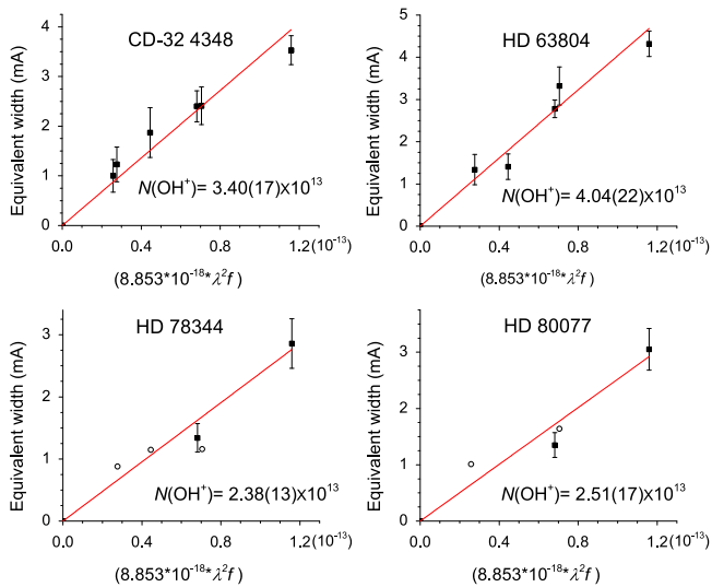
Figure 3. Weighted linear fits of measured equivalent widths to determine OH + column densities in the four translucent clouds studied here. Empty circles represent the tentatively detected lines that are not included in the fits.
