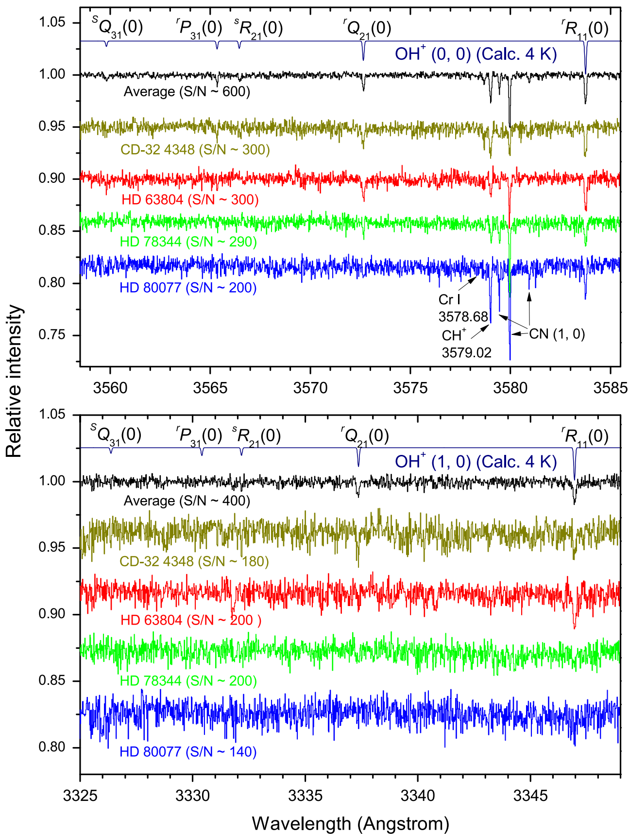
Figure 2. Spectra of the \text{OH}^+ \text{A}^3\Pi\text{-X}^3\Sigma^- (0, 0) and (1, 0) bands. From top to bottom in each panel: calculated 4 K spectrum, averaged spectrum, and individual spectra toward four high reddened stars. Spectra of the observed targets are normalized to pseudo-continuum, i.e., all broad features including stellar lines are eliminated for clarity. The narrow interstellar lines of \text{CH}^+ , Cr I, and CN are marked in the upper panel. The overall S/N estimated from the displayed wavelength regions are also presented for each spectrum.
