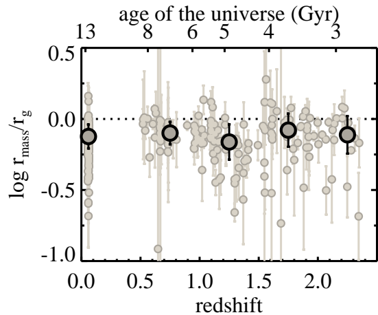
All galaxies
