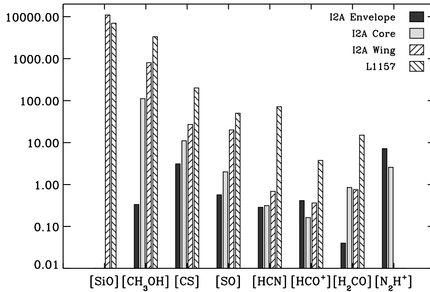
Figure 8.12. Abundances in the IRAS2A envelope (Jørgensen et al. 2004d) compared to the core and wing position components of the IRAS2A outflow (this paper) and the L1157 outflow (Bachiller & Pérez Gutiérrez 1997). The abundances have been normalized to the abundances of L134N. For SiO, which has not been detected in L134N, a “reference” abundance of 10^{-11} has been assumed. Note that N_2H^+ is not detected in the outflows, whereas SiO is not detected in the quiescent components.
