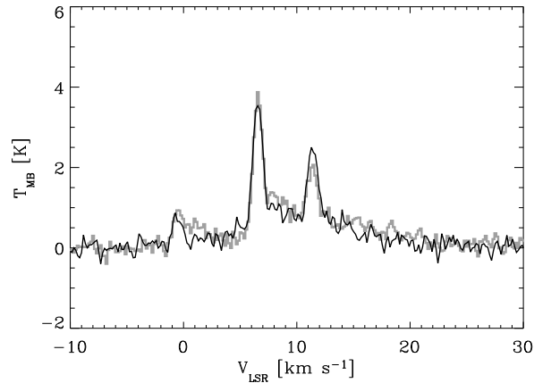
Figure 8.8. The HCN 1 – 0 spectrum toward the shock position (grey) overplotted with a composite of three versions of the HCO + spectrum toward the same position (black) - each shifted with the measured shifts between the HCN hyperfine lines and scaled according (relatively) to the 1:3:5 line-ratio expected for optically thin emission from material in LTE.
