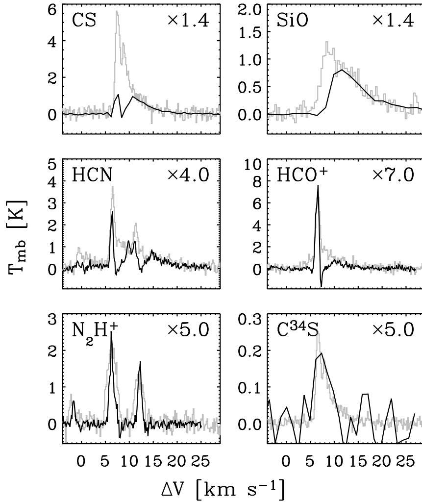
Figure 8.9. Comparison between the single-dish observations (grey) and corresponding spectra from the interferometer observations restored with the single-dish beam (black) at the shock position. The spectra from the interferometry observations have been scaled to resemble the wing of the single-dish spectra with the factors indicated in the upper right corner. For C ^{34} S the single-dish CS has been downscaled by a factor 22.
