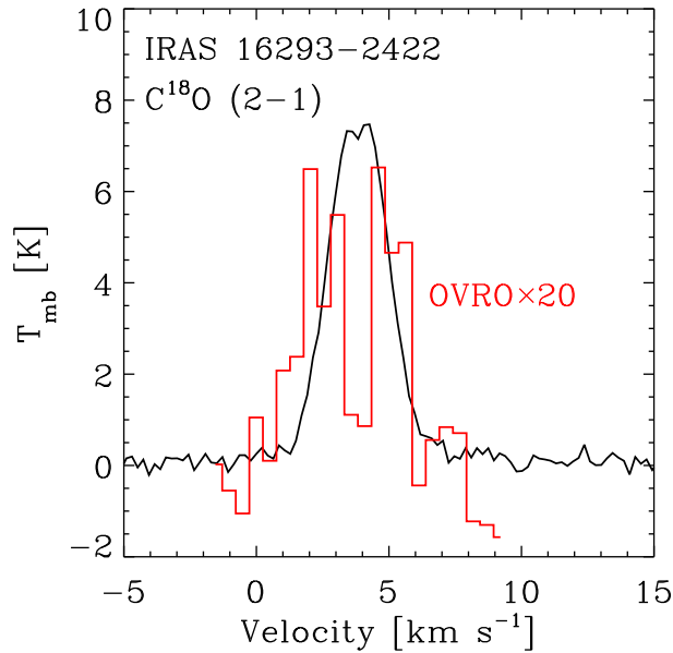
Figure 7.13. Comparison between the C 18 O J = 2 \rightarrow 1 line emission towards IRAS 16293–2422 at the source position, from JCMT single-dish observations (line diagram) and OVRO interferometric observations (histogram) restored with the JCMT beam (22"). The OVRO spectrum has been scaled in order to account for the flux seen in the JCMT spectrum.
