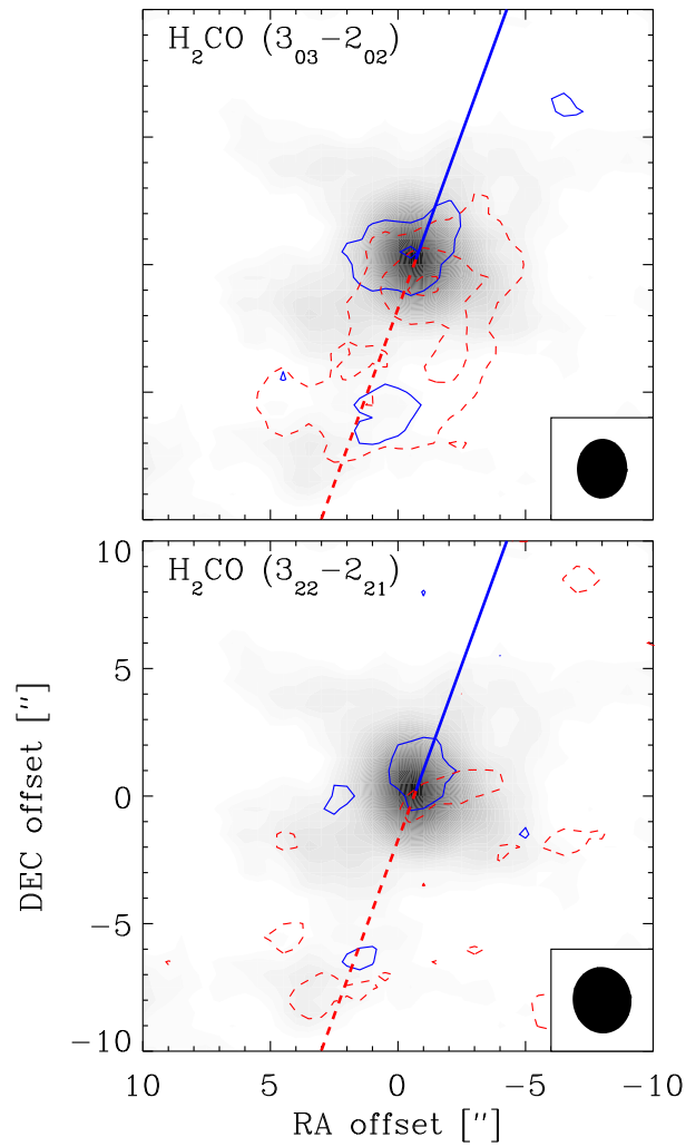
Figure 7.7. OVRO interferometer maps of H 2 CO emission (contours) overlaid on the 1.37 mm continuum emission (greyscale) for L1448-C. The H 2 CO emission has been separated into a red (dashed lines) and a blue (solid lines) part (see text for details). Contours start at 0.2 \text{ Jy beam}^{-1} \text{ km s}^{-1} ( 2\sigma ) and each successive contour is a multiple of this value. Also indicated are the directions of the large scale CO outflow.
