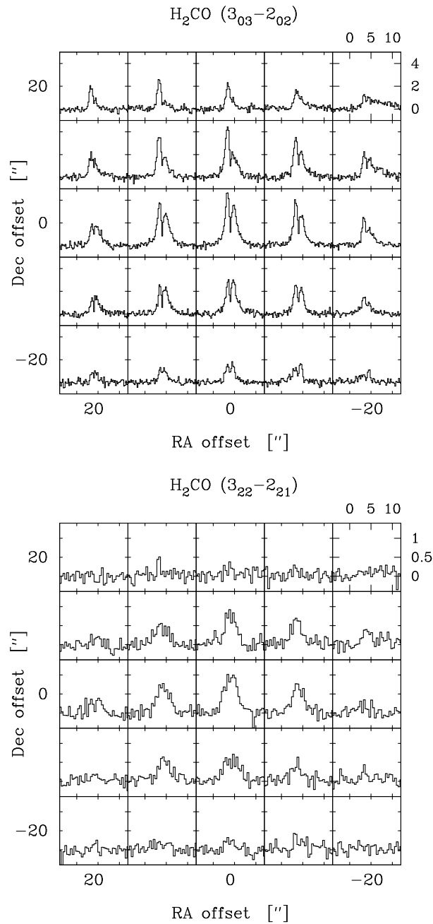
Figure 7.15. JCMT single-dish spectral maps of the H 2 CO emission toward IRAS 16293–2422. The velocity scale is in km s −1 and the intensity is the main beam brightness temperature in K as indicated in the upper right subplot. The spectral resolution is 0.22 km s −1 . The 3 22 → 2 21 line data have been smoothed to a two times lower spectral resolution.
