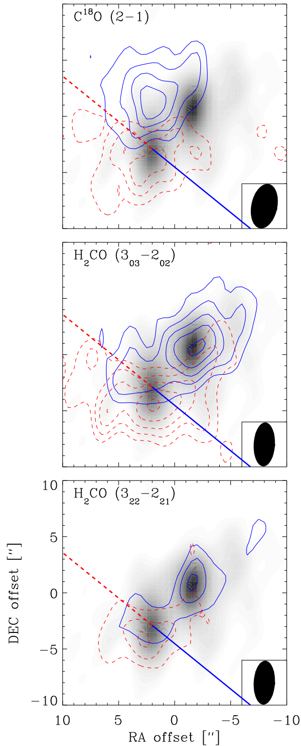
Figure 7.11. OVRO interferometer maps of IRAS 16293–2422 in C 18 O and H 2 CO line emission (contours) overlaid on the 1.37 mm continuum emission (greyscale). The molecular line emission has been separated into red (dashed lines) and blue (solid lines) components (see text for details). Contours start at 1.8 Jy beam -1 km s -1 for C 18 O and at 0.9 Jy beam -1 km s -1 for H 2 CO. The first contour corresponds to the '2σ'-level as estimated from the maps and each successive contour denotes an increase of 2σ. Also indicated is the direction of the large scale CO outflow.
