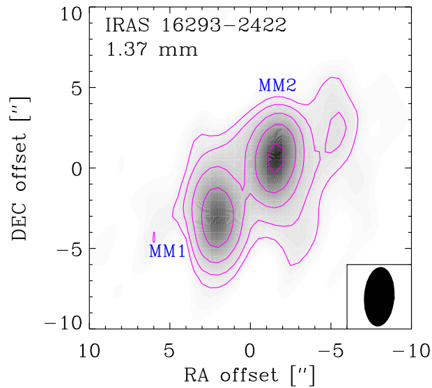
Figure 7.4. OVRO interferometer maps of the continuum emission at 1.37 mm towards IRAS 16293-2422. Contours start at 60 \text{ mJy beam}^{-1} and the first contour corresponds to the 2\sigma -level as estimated from the maps. Each successive contour is a multiple of two of the preceding value. The emission peaks at 0.82 and 1.1 \text{ Jy beam}^{-1} at MM1 and MM2, respectively.
