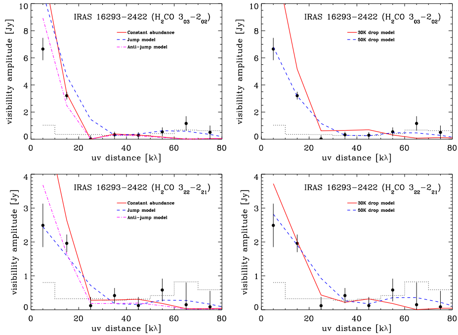
Figure 7.18. Visibility amplitudes of the observed H 2 CO line emission obtained at OVRO toward IRAS 16293–2422 as functions of the projected baseline length from the phase center, taken to be at (0''2, –1''2) for the common envelope. The observations, averaged over 1 to 7 km s –1 and binned to 10 kλ, are plotted as filled symbols with 1σ error bars. The dotted histogram represents the zero-expectation level. Also shown are the results of applying the same (u, v) sampling to the circumbinary envelope model using various H 2 CO abundance distributions. All models are consistent with available multi-transition single-dish data to within 3σ. See text and Fig. 7.10 for details on these models.
