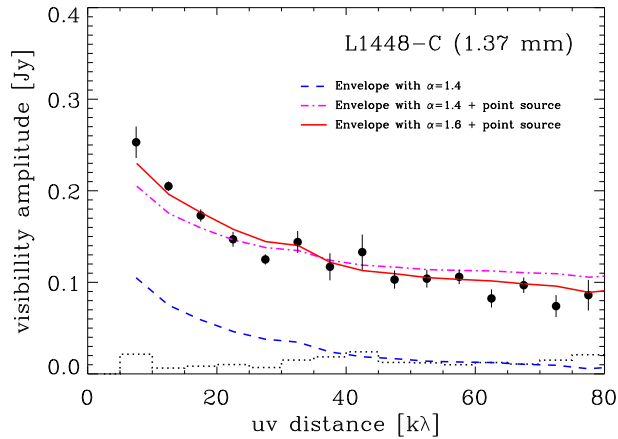
Figure 7.2. Visibility amplitudes of the observed 1.37 mm continuum emission obtained at OVRO towards L1448-C as functions of the projected baseline length, binned to 5 k\lambda , from the phase center, taken to be at (-0''.6, 0''.2) . The observations are plotted as filled symbols with 1\sigma error bars. The dotted histogram represents the zero-expectation level. Also shown are predictions based on a realistic physical model for the source (Jørgensen et al. 2002), with the same (u, v) sampling as the observations (see text for details). Unresolved compact emission, presumably from a circumstellar disk, must be added to that from the envelope to produce an acceptable fit.
